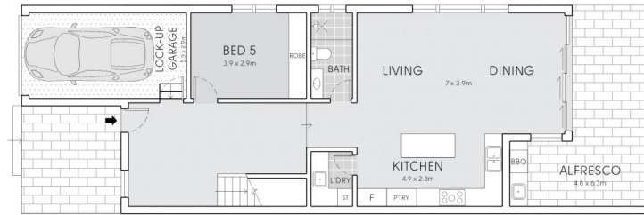
GROUND FLOOR
