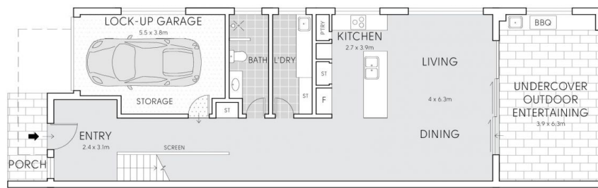
GROUND FLOOR
