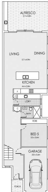
GROUND FLOOR
