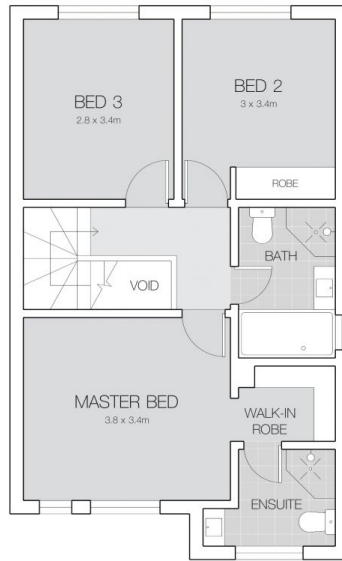
LEVEL ONE
