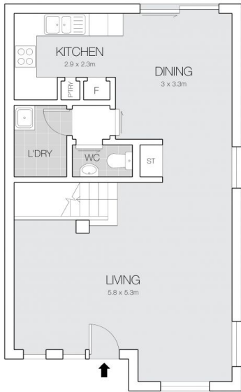
GROUND LEVEL
