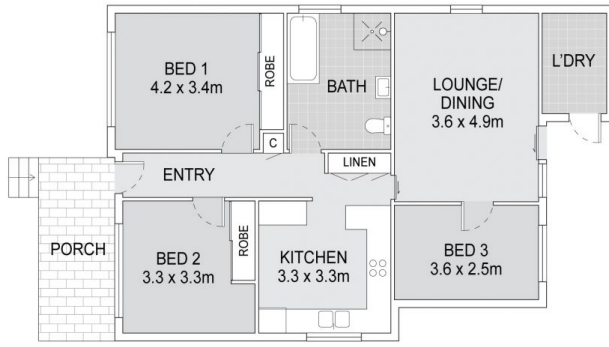
MAIN HOUSE
