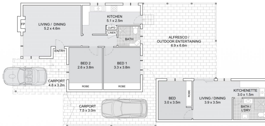
SITE PLAN
